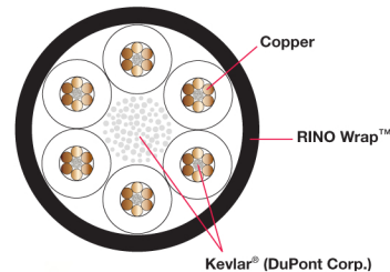
Illustration of typical RINO ™ cable (cross section)
