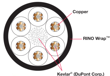
Illustration of typical RINO™ cable (cross section)
